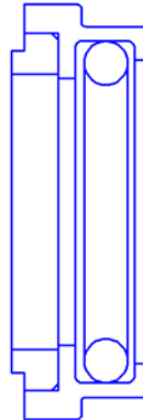
SEAL CASE WITH O-RING
