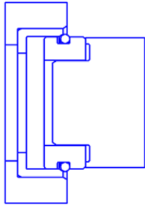
INSTALLING MAGNET INTO INSULATOR USING DRIFT
