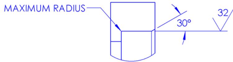
Magnet Bore Radius and Lead Chamfer
